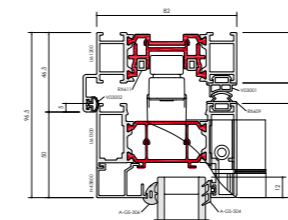
F82 Head
