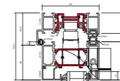
F82 Head
